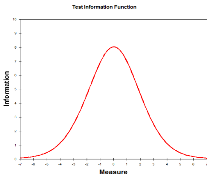
Graph 1. Tes Information Function
