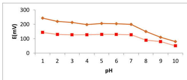
29 Figure 2. Effect of pH on Potential response of ISE-La(III)
